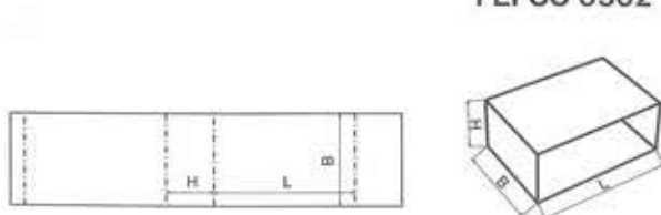
FEFCO 0502
