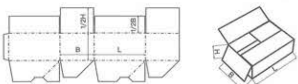
FEFCO 0713
