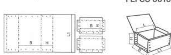
FEFCO 0610
