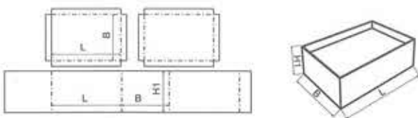
FEFCO 0620
