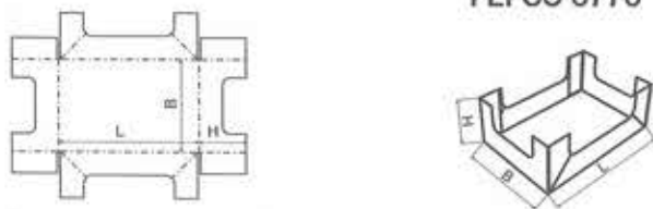
FEFCO 0770
