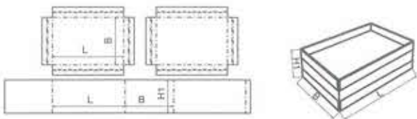
FEFCO 0616
