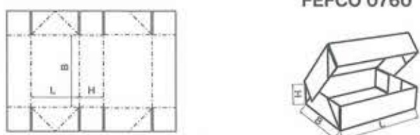
FEFCO 0761
