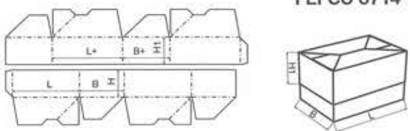
FEFCO 0714
