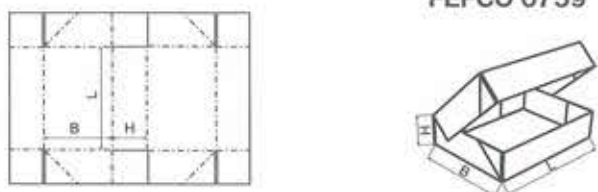
FEFCO 0760
